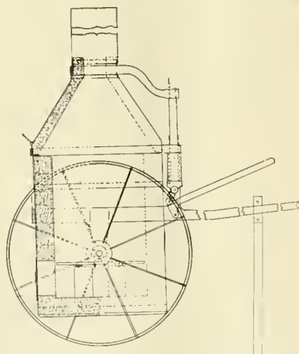
PORTABLE FURNACE FOR BRONZE OR BABBITT.
